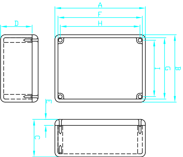
DETAILED DIMENSION IN mm
